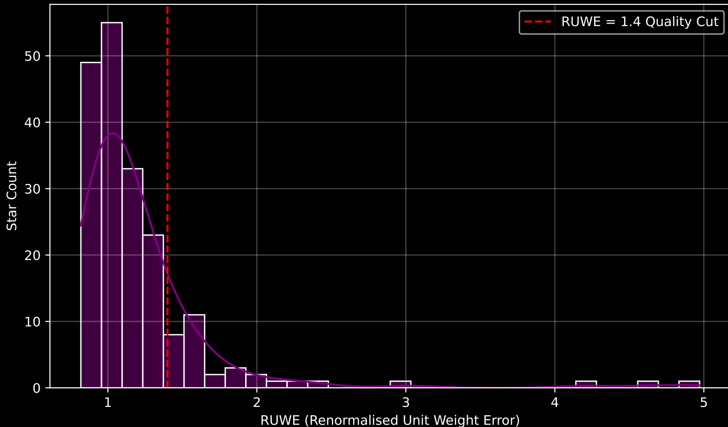
GALAH DR4 Field [6783] RUWE Distribution (n= 193)
