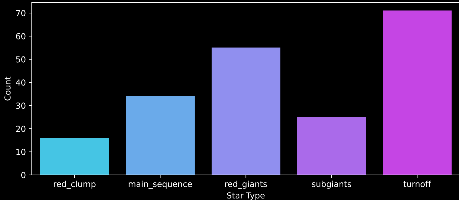
GALAH DR4 Field: [6783] Count plot of Star Type
