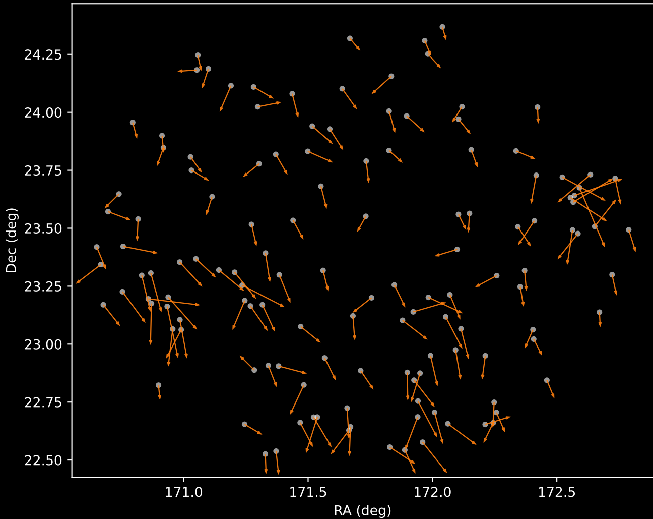
GALAH DR4 Cluster 2 Proper Motion Vectors (n=133)
