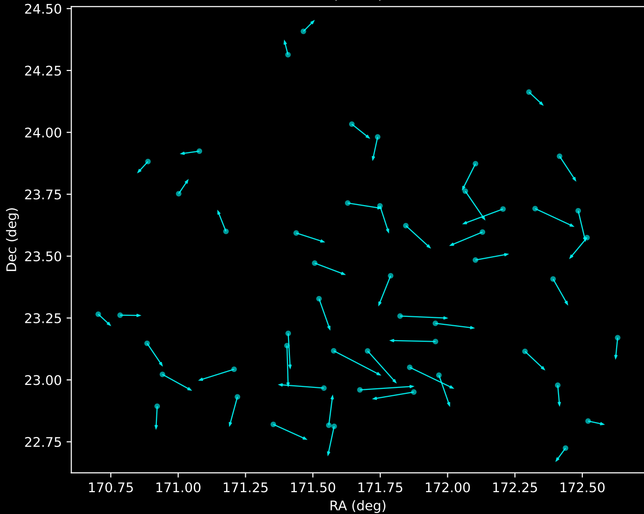
GALAH DR4 Noise Stream Proper Motion Vectors (n=53)
