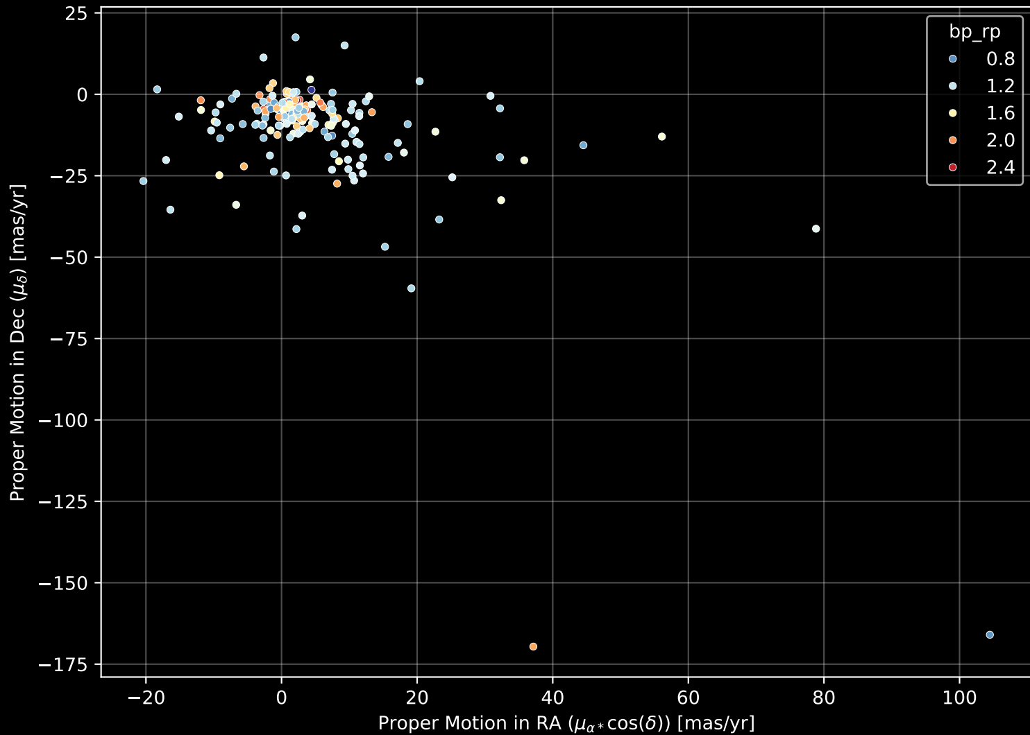
GALAH DR4 Field: [6783] Proper Motion Diagram (n= 201)
